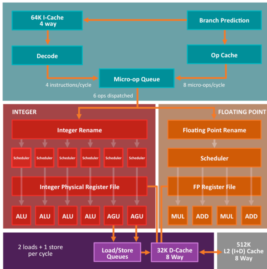
Figure 1. Zen CPU microarchitecture. The branch predictor and micro-op cache provide a significant performance boost. (Source: AMD)
