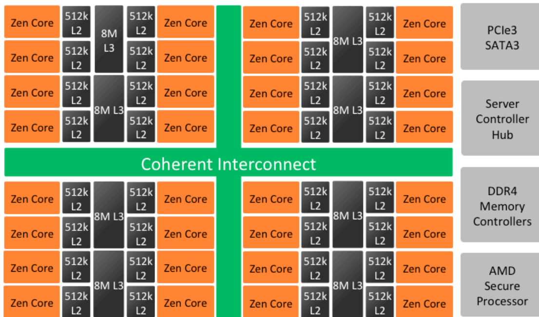
Figure 2. EPYC processor design. The coherent interconnect links up to 32 CPU cores in clusters of four, each with its own 8MB level-three cache. (Source: AMD)
