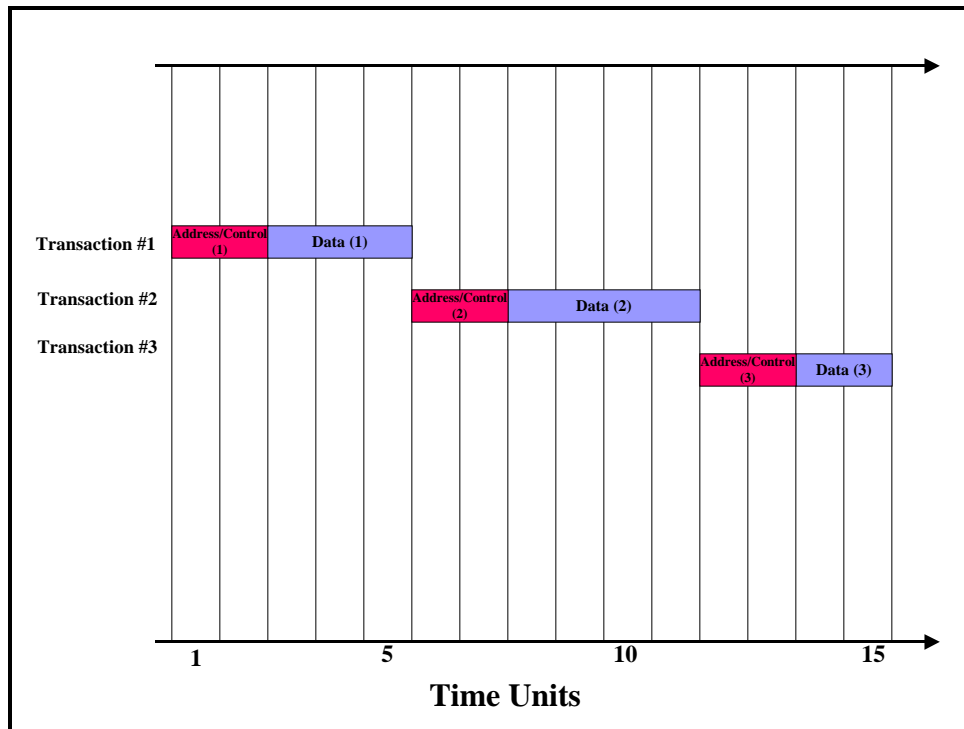
Figure 6: Example of Serialized Transaction Nature of Non-Split Transaction Bus Architectures
