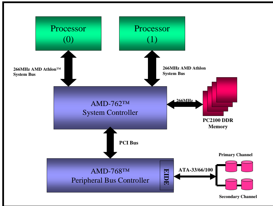
Figure 15: The AMD-760™ MPX Chipset EIDE Controller Supporting ATA-33/66/100MB/s Speeds
