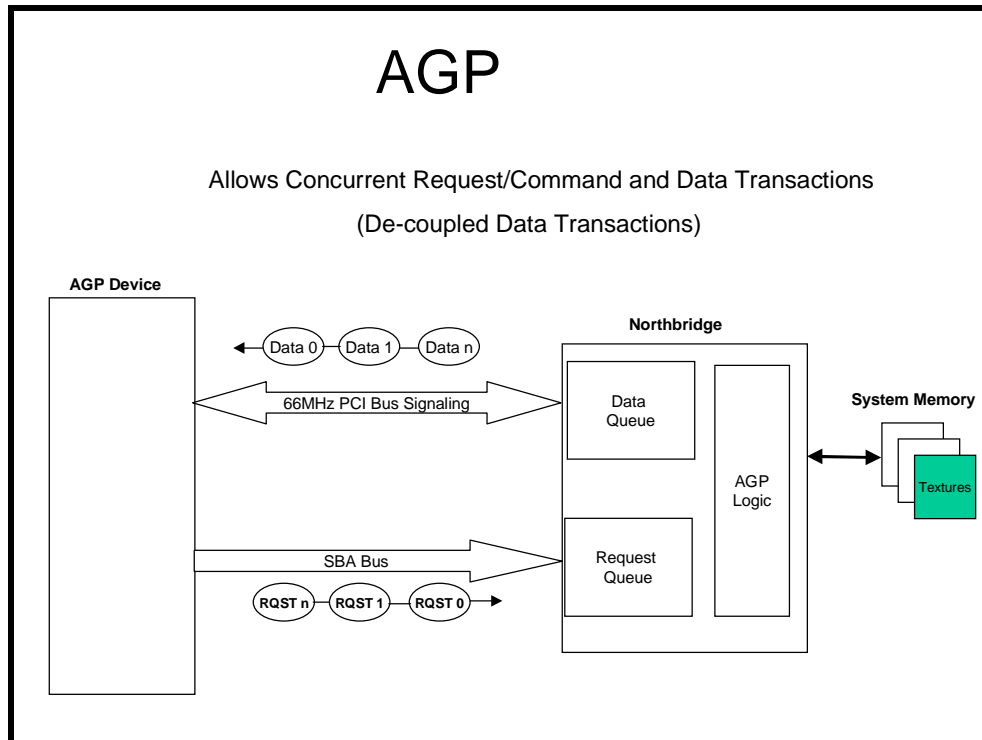
Figure 20: High-Level AGP Interface Diagram Showing Bus Architecture and Embedded Northbridge Components
