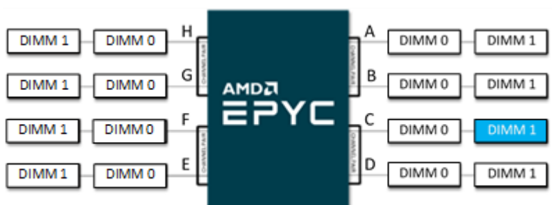
Figure 2. One DIMM Population in 2 DPC Configuration
