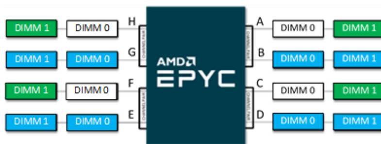
Figure 12. Example Twelve DIMM Population in 2 DPC Configuration
