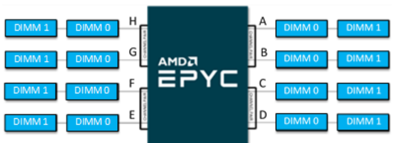
Figure 14. Example Sixteen DIMM Population in 2 DPC Configuration
