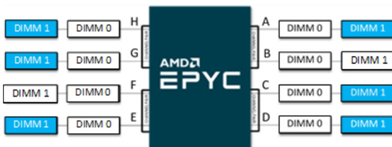
Figure 8. Example Six DIMM Population in 2 DPC Configuration
