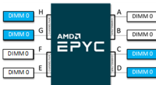
Figure 5. Example Four DIMM Population in 1 DPC Configuration
