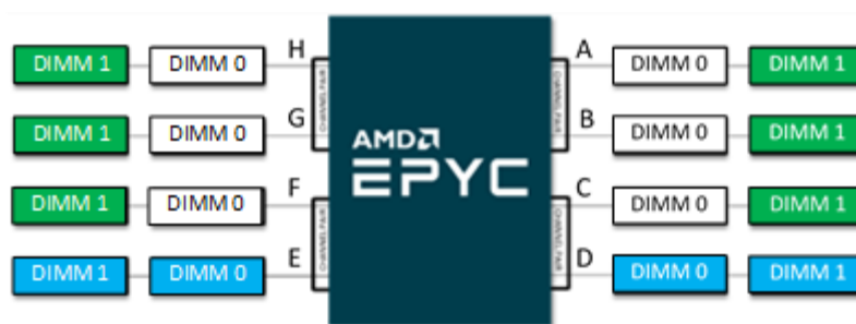
Figure 11. Example Ten DIMM Population in 2 DPC Configuration
