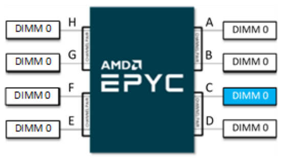
Figure 1. One DIMM Population in 1 DPC Configuration
