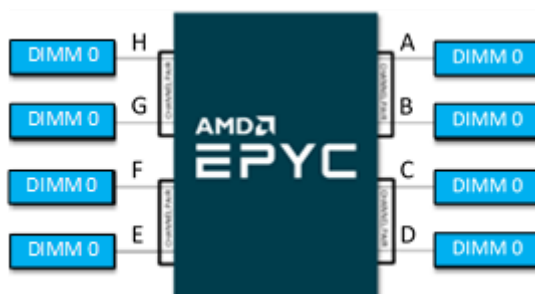
Figure 9. Example Eight DIMM Population in 1 DPC Configuration
