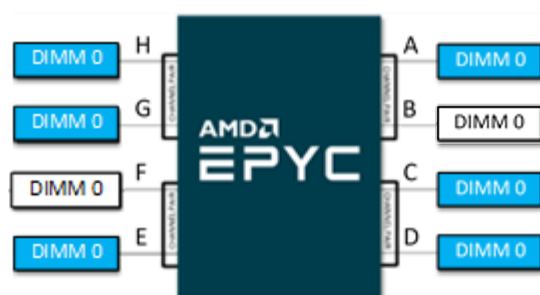
Figure 7. Example Six DIMM Population in 1 DPC Configuration
