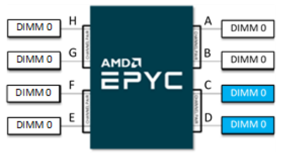
Figure 3. Example Two DIMM Population in 1 DPC Configuration
