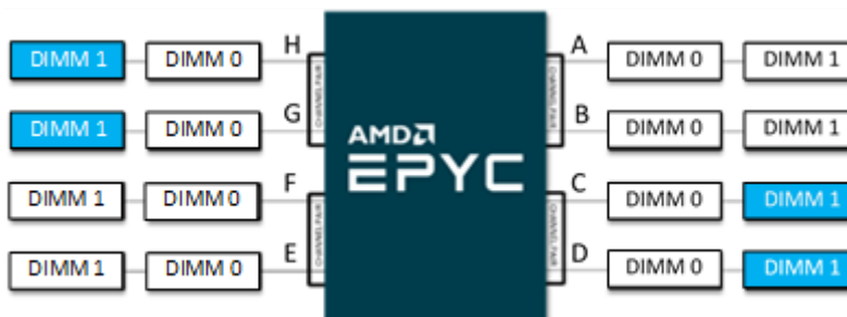
Figure 6. Example Four DIMM Population in 2 DPC Configuration
