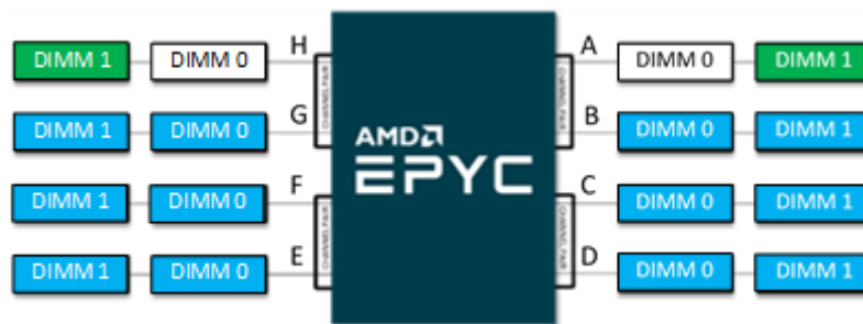
Figure 13. Example Fourteen DIMM Population in 2 DPC Configuration
