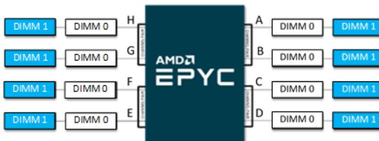
Figure 10. Example Eight DIMM Population in 2 DPC Configuration
