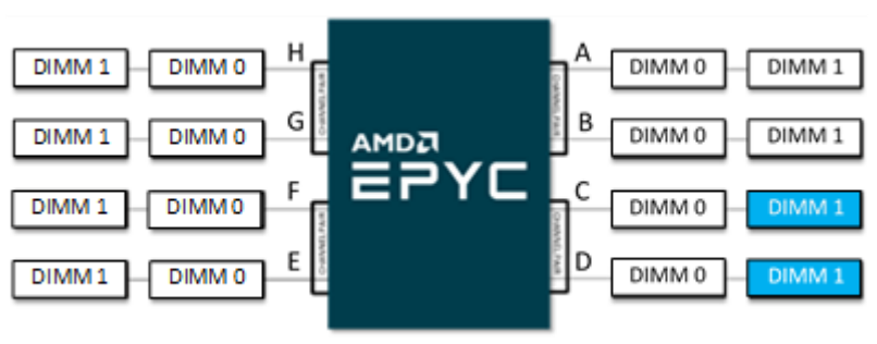
Figure 4. Example Two DIMM Population in 2 DPC Configuration
