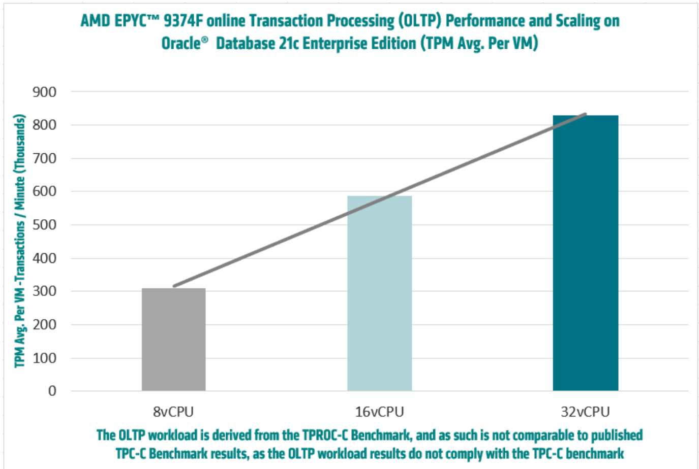
Figure 1 AMD EPYC 9374F OLTP performance scaling on Oracle 21c Enterprise Edition on two sockets, 4 host Nutanix NX servers.
