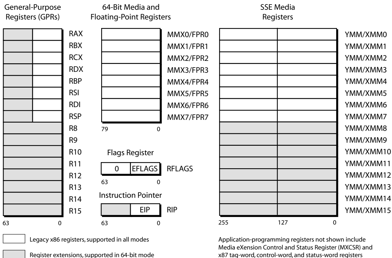
Figure 1-1. Application-Programming Register Set
