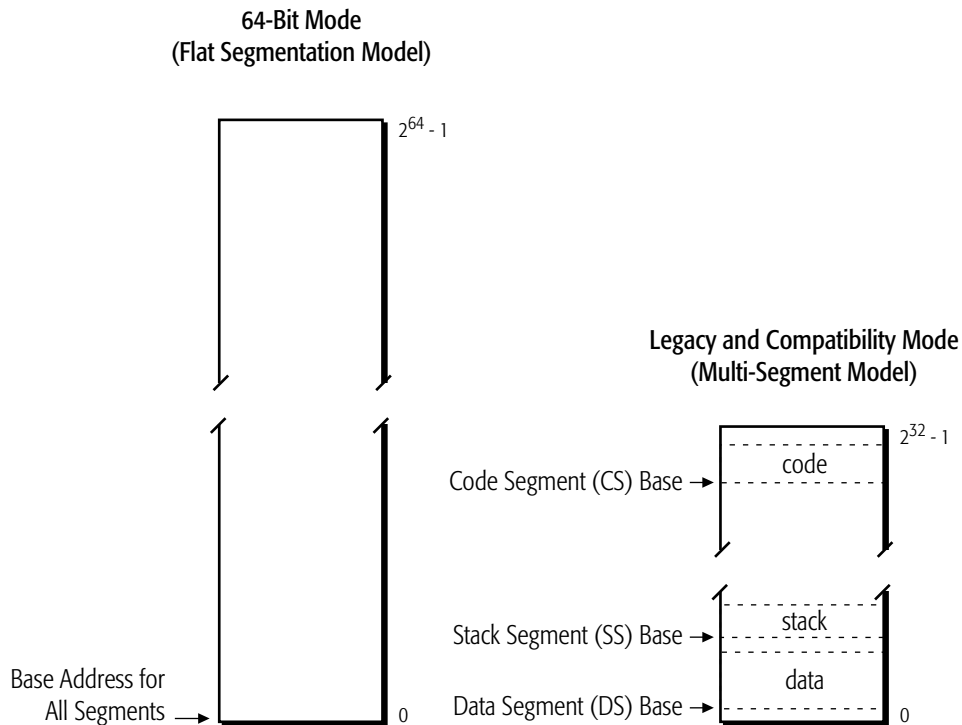
Figure 2-1. Virtual-Memory Segmentation
