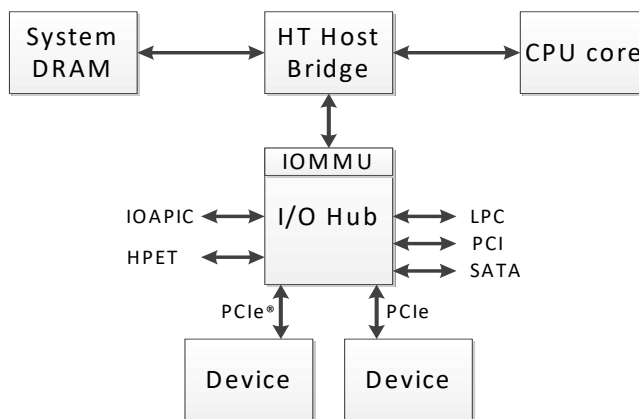
Figure 88: Example Platform Architecture
