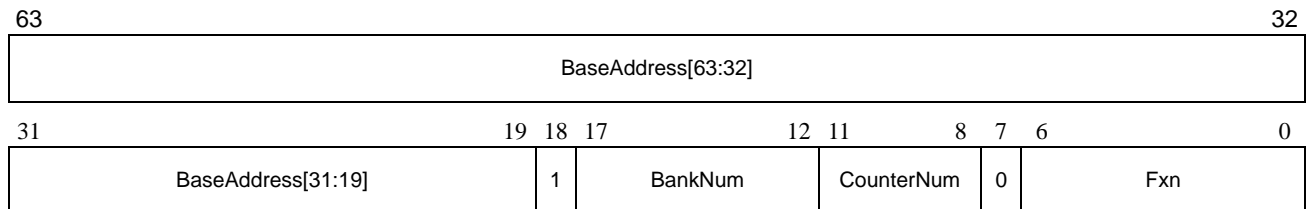
Figure 83: IOMMU Counter Register Address Decode
