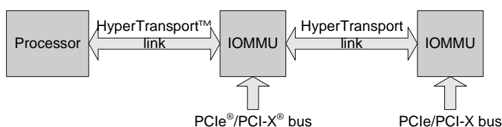
Figure 87: Chained Hybrid IOMMU in a Large System
