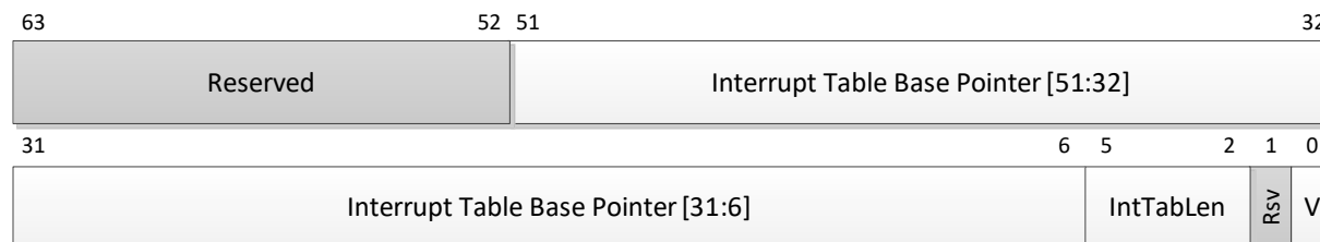
Figure 82: Level-1 Interrupt Table Entry Format
