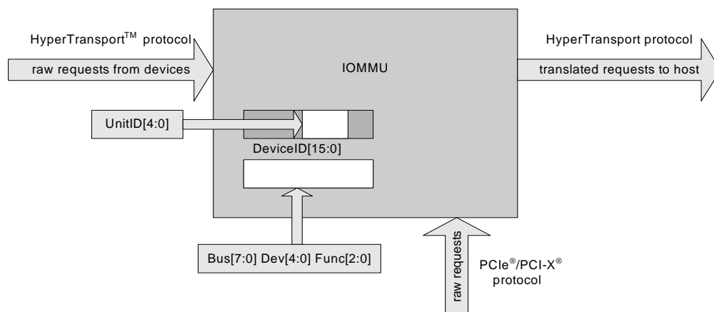
Figure 86: Hybrid IOMMU
