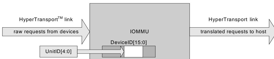
Figure 84: IOMMU in a Tunnel
