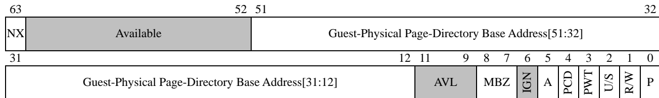
Figure 28: AMD64 Long Mode 4-Kbyte PDPE Format
