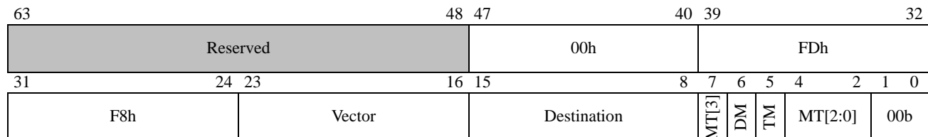
Figure 3: System Management Interrupt Address Format
