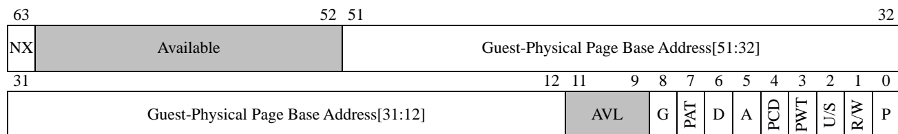
Figure 30: AMD64 Long Mode 4-Kbyte PTE Format
