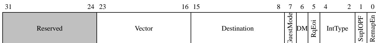
Figure 15: Interrupt Remapping Table Entry - Basic Format
