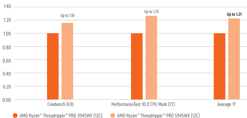
FIGURE 6: 1T TEST RESULTS FOR 2ND GENERATION 12C AMD THREADRIPPER™ PRO 5945WX, NORMALIZED TO 1ST GENERATION 12C 3945WX, ON SIMILARLY CONFIGURED SYSTEM. 5,6
