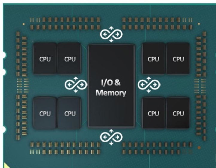
FIGURE 2: AMD INFINITY FABRIC™ ENABLES THREADRIPPER™ PRO PROCESSORS’ CHIPLET IMPLEMENTATION, PROVIDING AN OUTSTANDING COMBINATION OF CORES RUNNING AT HIGH CLOCK RATES (SEE FIGURE 5).
