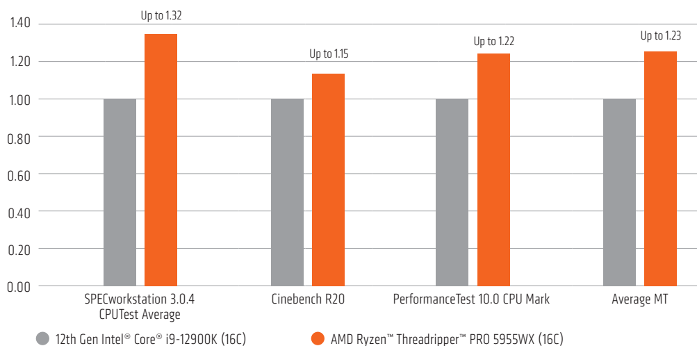
FIGURE 13: MULTI-THREADED CPU-SPECIFIC TEST RESULTS FOR THE 16C THREADRIPPER™ PRO 5955WX, NORMALIZED TO THE 16C INTEL CORE i9-12900K, WITH SIMILARLY CONFIGURED SYSTEMS 6 , NORMALIZED TO 12TH GEN INTEL® CORE® i9-12900K (16C)
