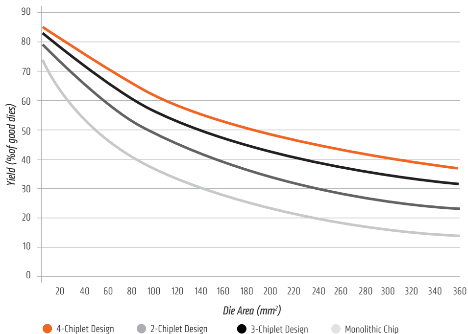
FIGURE 5: CHIPLET APPROACHES LIKE AMD INFINITY ARCHITECTURE PROVIDE FOR SUPERIOR SCALING (SOURCE: WIKICHIP)
