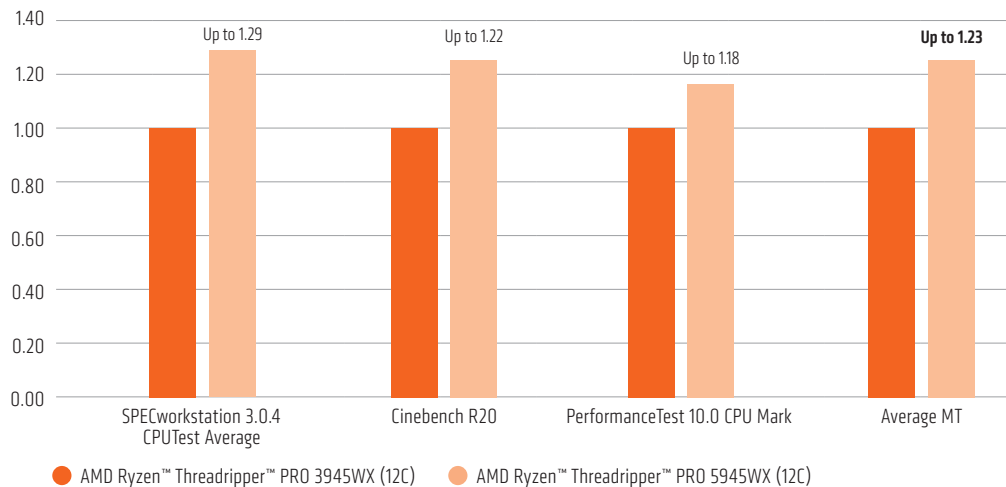
FIGURE 7: MULTI-THREAD (MT) GENERATION-TO-GENERATION 12C TEST RESULTS FOR SIMILARLY CONFIGURED SYSTEMS 5,6 , NORMALIZED TO AMD THREADRIPPER PRO 3945WX
