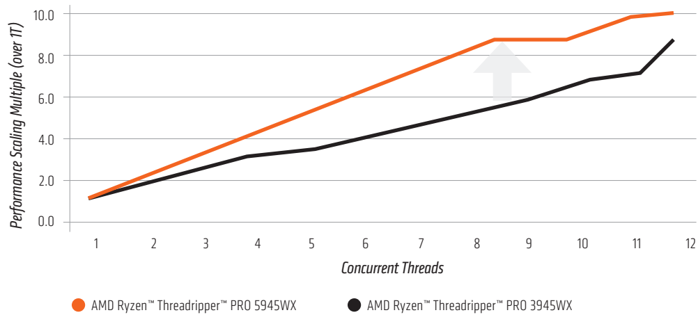
FIGURE 9: MULTI-THREAD (MT) TEST RESULTS SHOWING EACH GENERATION'S 12C CPU PERFORMANCE SCALING MULTIPLE (OVER ITS OWN 1T SCORE) RUNNING PASSMARK PERFORMANCETEST 10'S COMPRESSION TEST ON SIMILARLY CONFIGURED SYSTEMS 5,6
