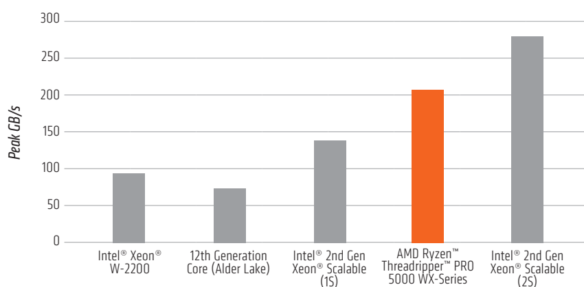
FIGURE 6: AMD RYZEN™ THREADRIPPER™ PRO 5000 WX-SERIES PROCESSORS WITH 8 CHANNELS OF DDR4-3200 ECC MEMORY OFFER MORE MAXIMUM MEMORY BANDWIDTH THAN ANY WORKSTATION CPU IN A SINGLE SOCKET AVAILABLE TODAY (SOURCE: AMD AND INTEL)
