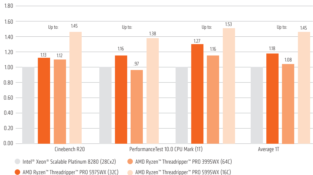
FIGURE 14: MULTI-THREAD TEST RESULTS FOR SIMILARLY CONFIGURED SYSTEMS 8 , NORMALIZED TO INTEL® XEON® SCALABLE PLATINUM 8280 (28CX2)
