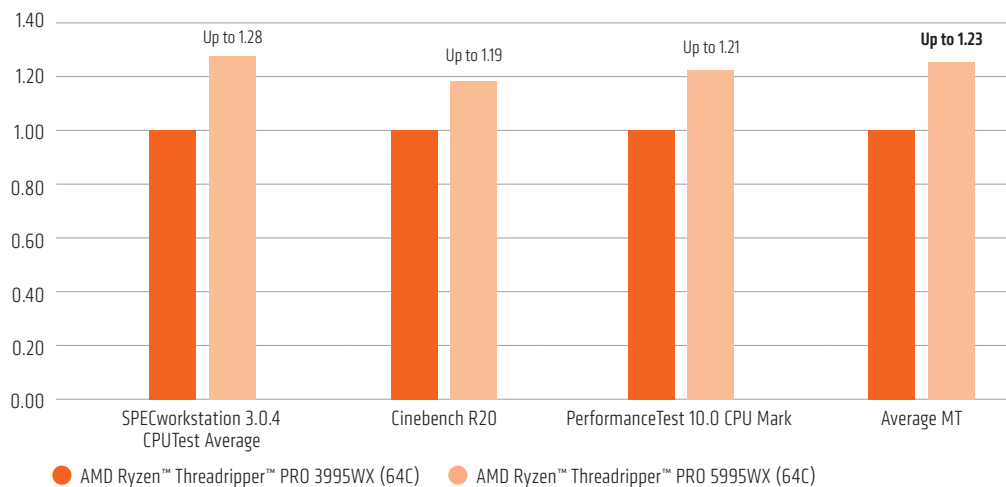
FIGURE 8: MULTI-THREAD (MT) GENERATION-TO-GENERATION 64C TEST RESULTS FOR SIMILARLY CONFIGURED SYSTEMS 5,6 , NORMALIZED TO AMD THREADRIPPER PRO 3995WX
