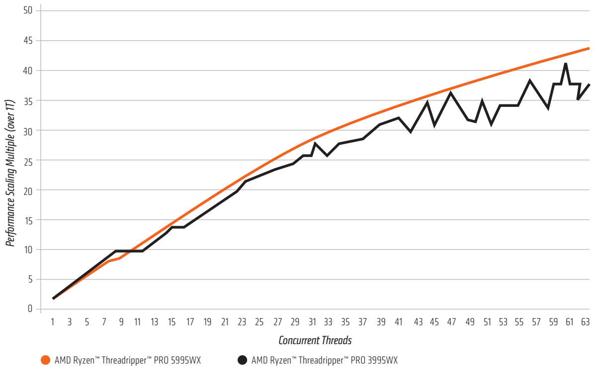
FIGURE 10: MULTI-THREAD (MT) TEST RESULTS SHOWING EACH GENERATION'S 64C CPU'S PERFORMANCE SCALING MULTIPLE (OVER ITS OWN 1T SCORE) RUNNING PASSMARK PERFORMANCETEST 10'S COMPRESSION TEST ON SIMILARLY CONFIGURED SYSTEMS ii,iii
