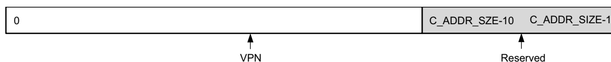
Figure 2-17: TLBSX
