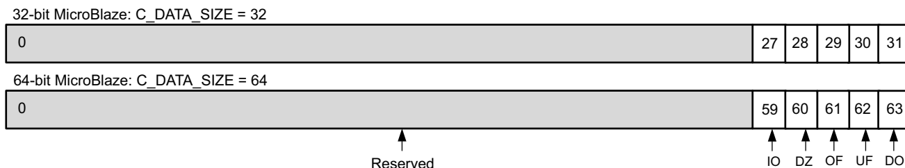
Figure 2-8: FSR
