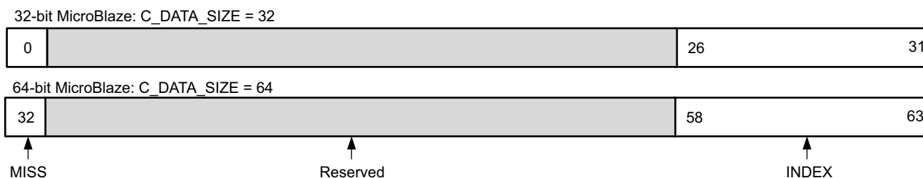
Figure 2-16: TLBX
