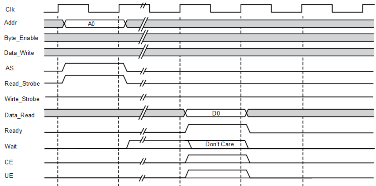
Figure 3-7: LMB Generic Read Operation, N Wait States
